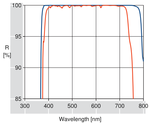
BROADBAND H.R. COATING R55: 425-675nm S-POL, 45° ———— P-POL, 45° ————
