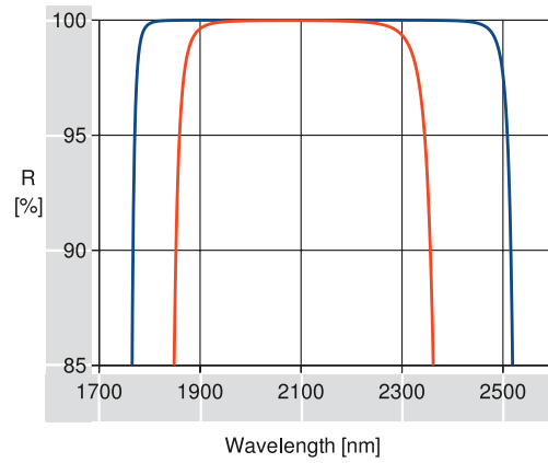
NARROWBAND H.R. COATING R50: 2060-2100nm S-POL, 45° ———— P-POL, 45° ————
