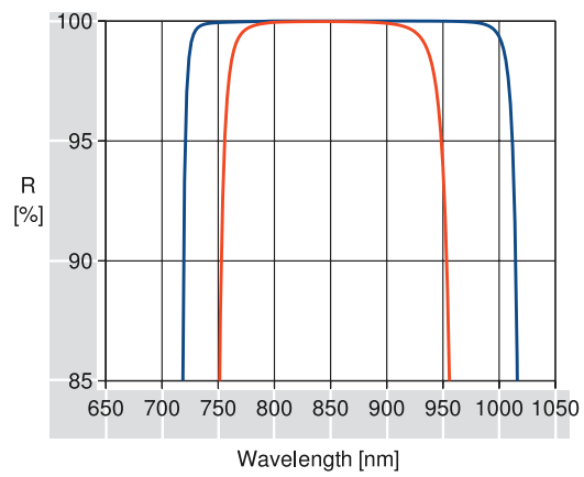
NARROWBAND H.R. COATING R42: 780-905nm S-POL, 45° ———— P-POL, 45° ————
