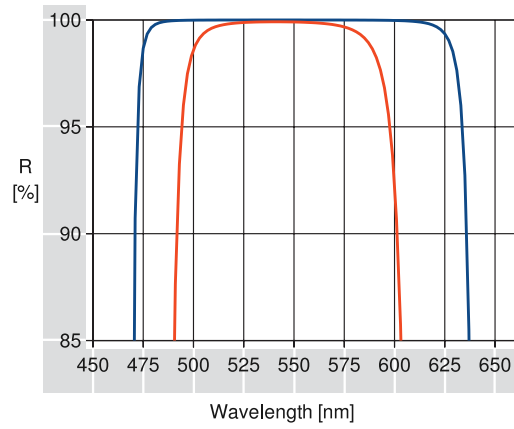
NARROWBAND H.R. COATING R28: 543nm S-POL, 45° ———— P-POL, 45° ————
