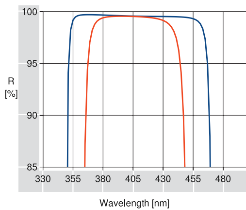
NARROWBAND H.R. COATING R16: 405nm S-POL, 45° ——— P-POL, 45° ———
