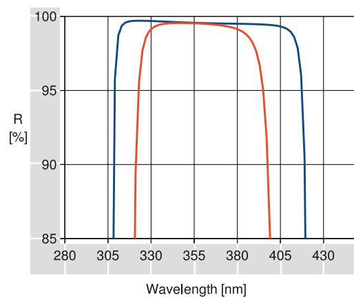
NARROWBAND H.R. COATING R14: 355nm S-POL, 45° ———— P-POL, 45° ————
