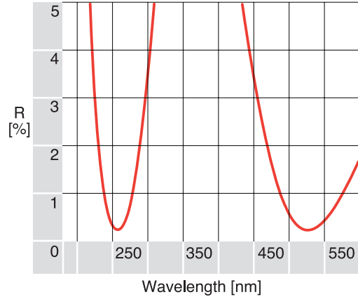
MULTIBAND ANTI-REFLECTION COATING A79 (266 & 532 nm) —
