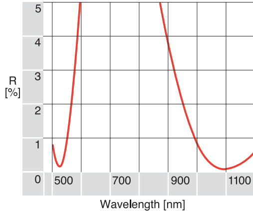
MULTIBAND ANTI-REFLECTION COATING A78 (532 & 1064 nm) ———
