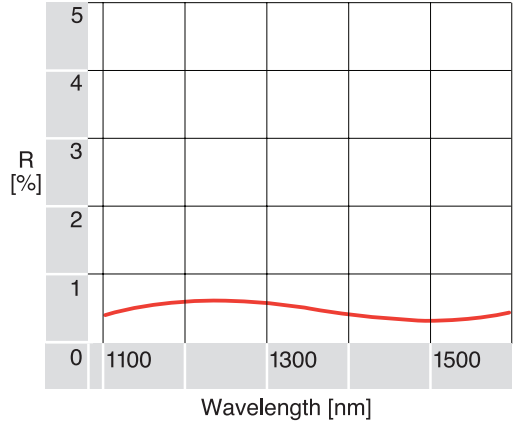
NEAR IR BROADBAND ANTI-REFLECTION COATING A67 (1100-1600 nm) —
