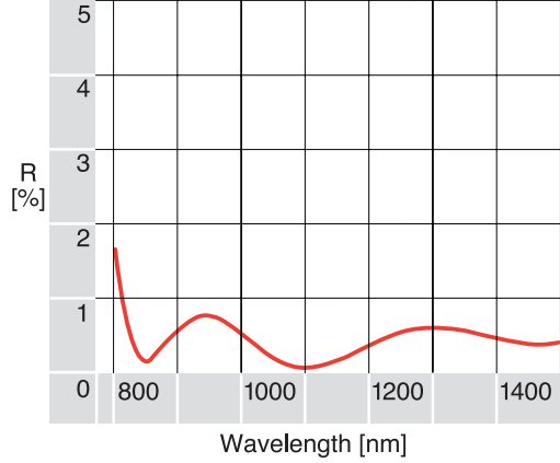
NEAR IR BROADBAND ANTI-REFLECTION COATING A63 (850-1500 nm) —
