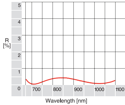
NEAR IR BROADBAND ANTI-REFLECTION COATING A62 (670-1100nm)
