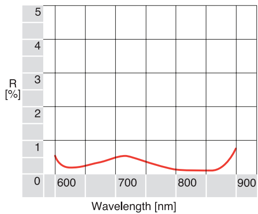
VISIBLE/NEAR IR BROADBAND ANTI-REFLECTION COATING A58 (600-900 nm) ———
