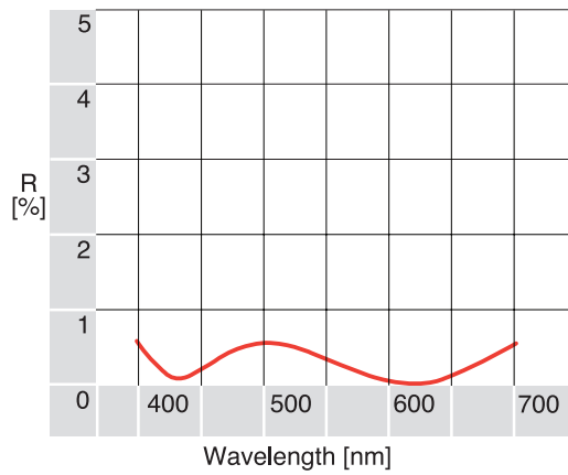
VISIBLE BROADBAND ANTI-REFLECTION COATING A55 (425-675nm) ———
